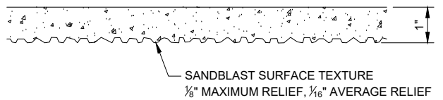
DETAIL ROUGHENED FINISH
