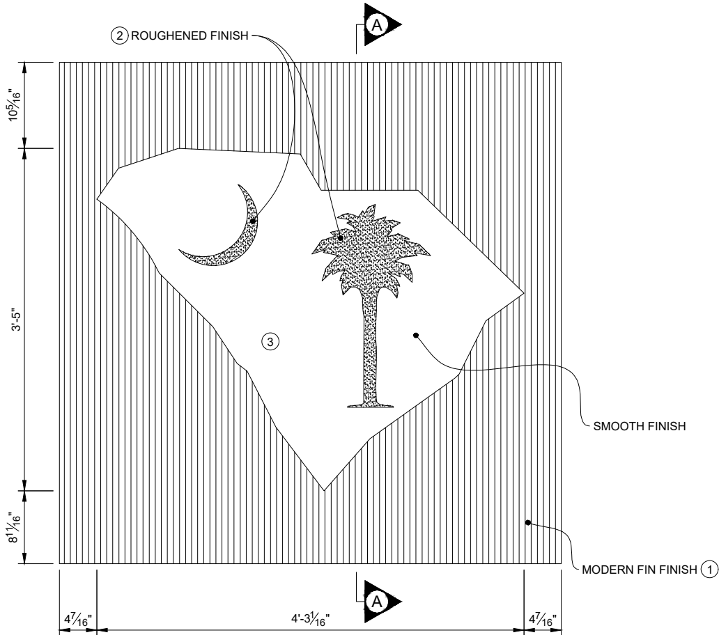
DETAIL MSE WALL PANEL WITH INLAY (ELEVATION) 1
