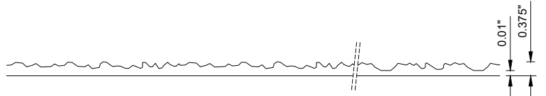
SECTION B MODERN FIN FINISH
