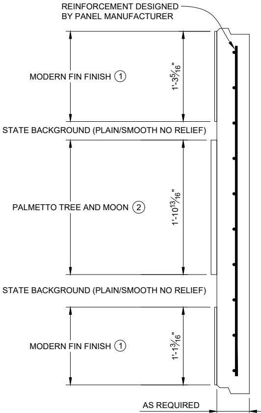
SECTION MSE WALL PANEL WITH INLAY
