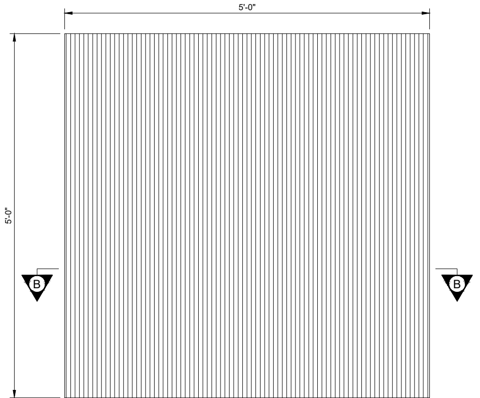
DETAIL MSE WALL PANEL MODERN FIN FINISH (ELEVATION) 2
