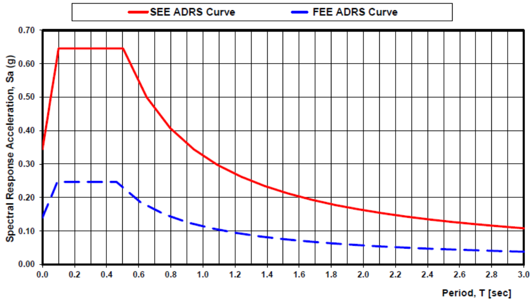
SC Seismic Hazard Map Three-Point ADRS Curve From Ground Surface, SC 769 - Site Class C
