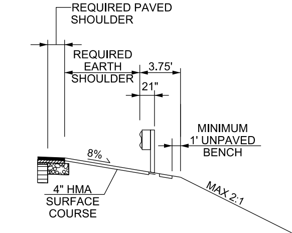
STANDARD GUARDRAIL DETAIL WITH ASPHALT NON-MOW STRIP
