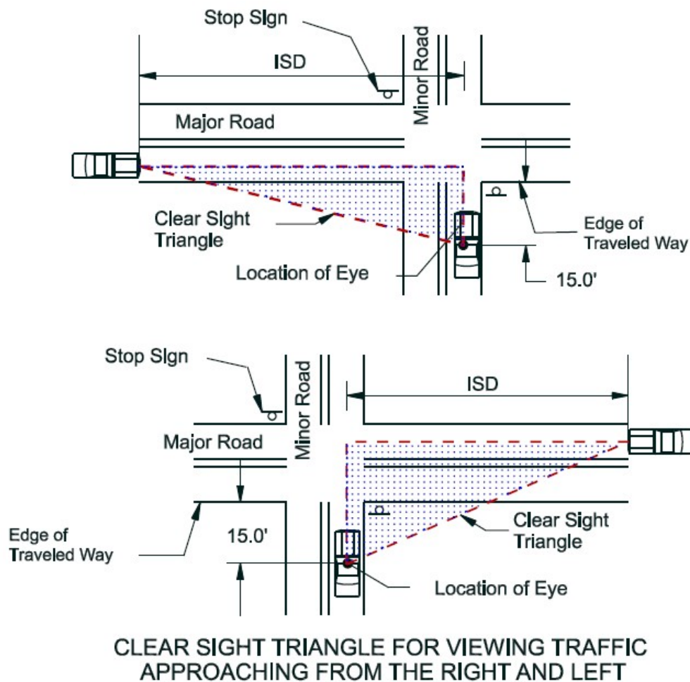
Figure 7-23: Sight Triangles
