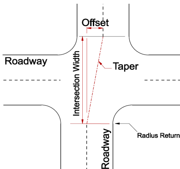
Figure 5-20: Offset Intersection Legs
