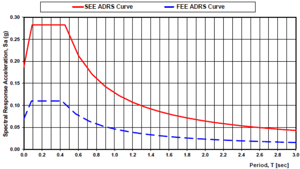
SC Seismic Hazard Map Three-Point ADRS Curve From Ground Surface, S-20-101 - Site Class C
