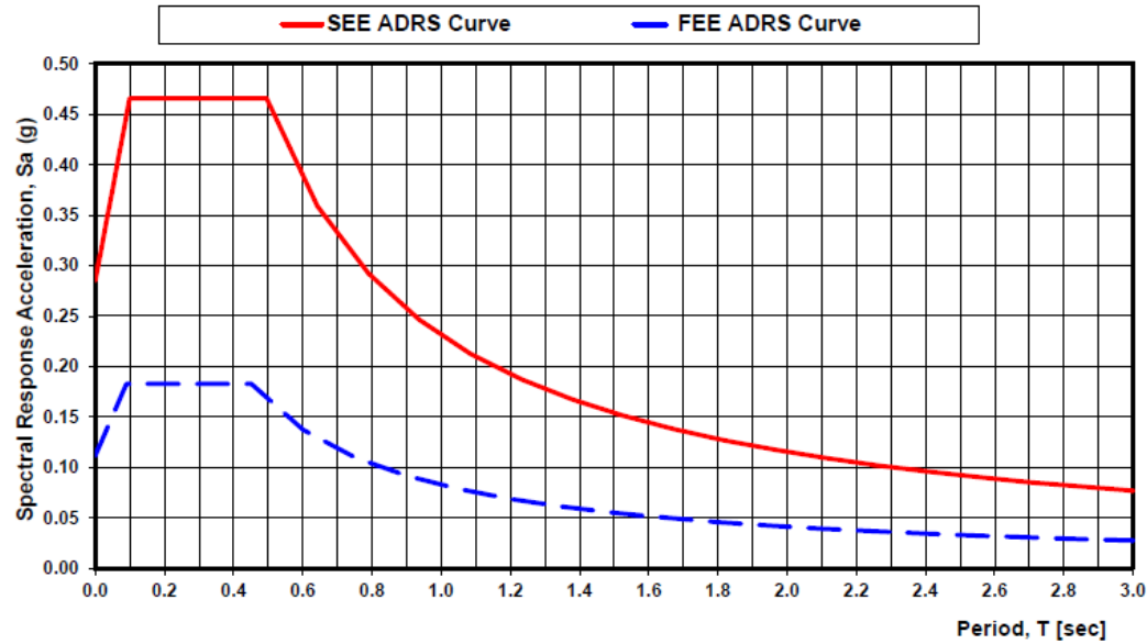
SC Seismic Hazard Map Three-Point ADRS Curve From Ground Surface
