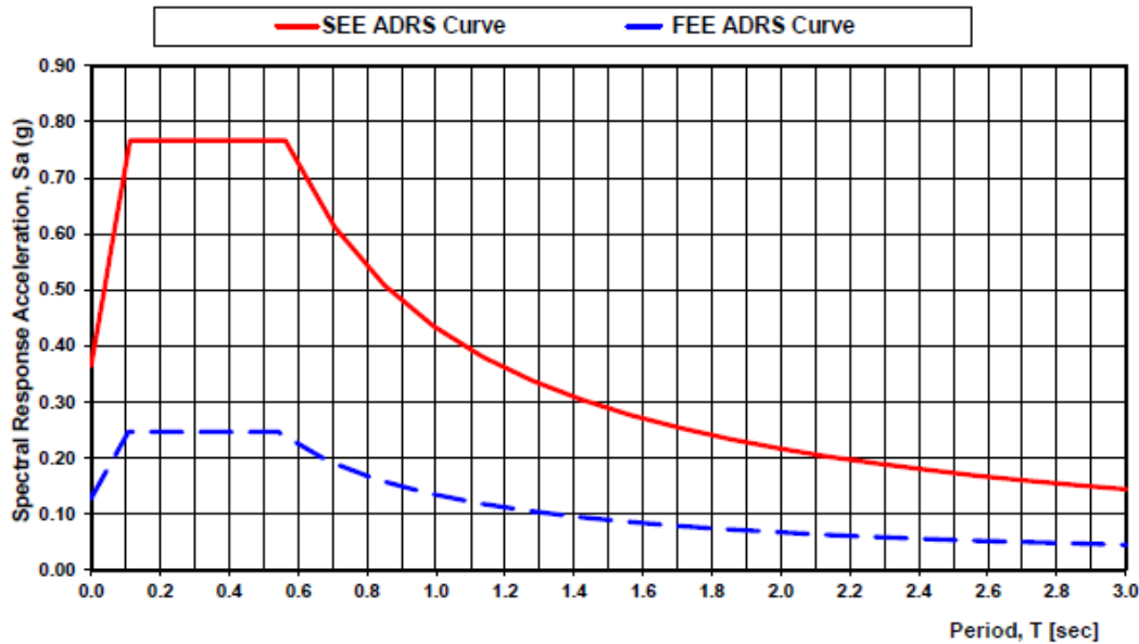
SC Seismic Hazard Map Three-Point ADRS Curve From Ground Surface, S-21-57 - Site Class D
