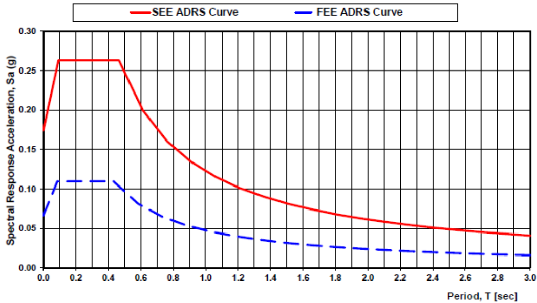
SC Seismic Hazard Map Three-Point ADRS Curve From Ground Surface, SC 34 - Site Class C
