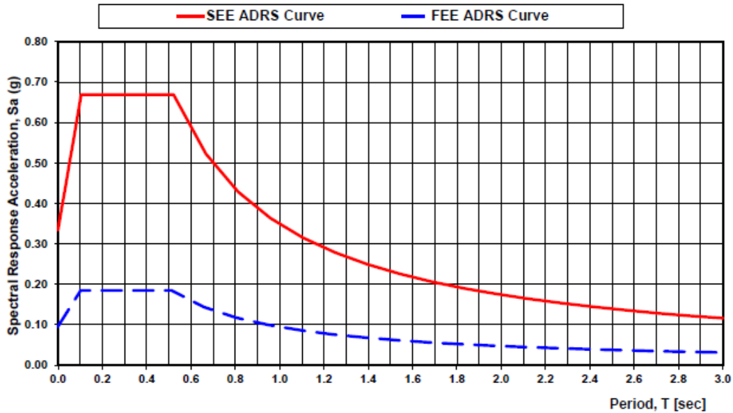
SC Seismic Hazard Map Three-Point ADRS Curve From Ground Surface, S-21-57 - Site Class C
