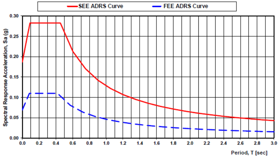
SC Seismic Hazard Map Three-Point ADRS Curve From Ground Surface, S-20-101 - Site Class C
