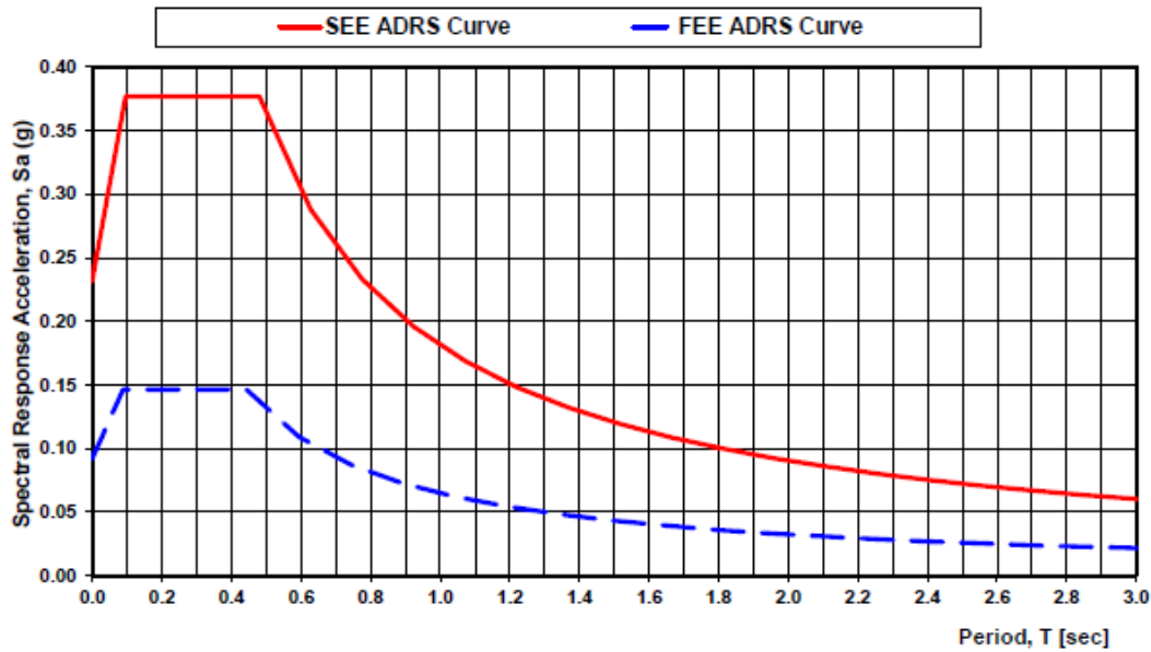
SC Seismic Hazard Map Three-Point ADRS Curve From Ground Surface, S-20-101 - Site Class D
