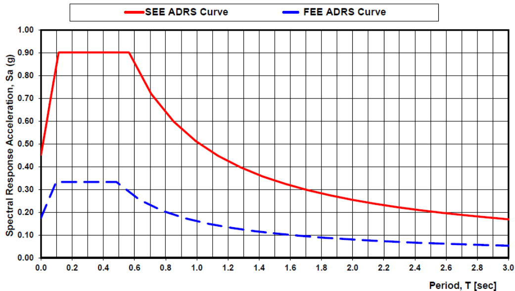
SC Seismic Hazard Map Three-Point ADRS Curve From Ground Surface, US 301 - Site Class D
