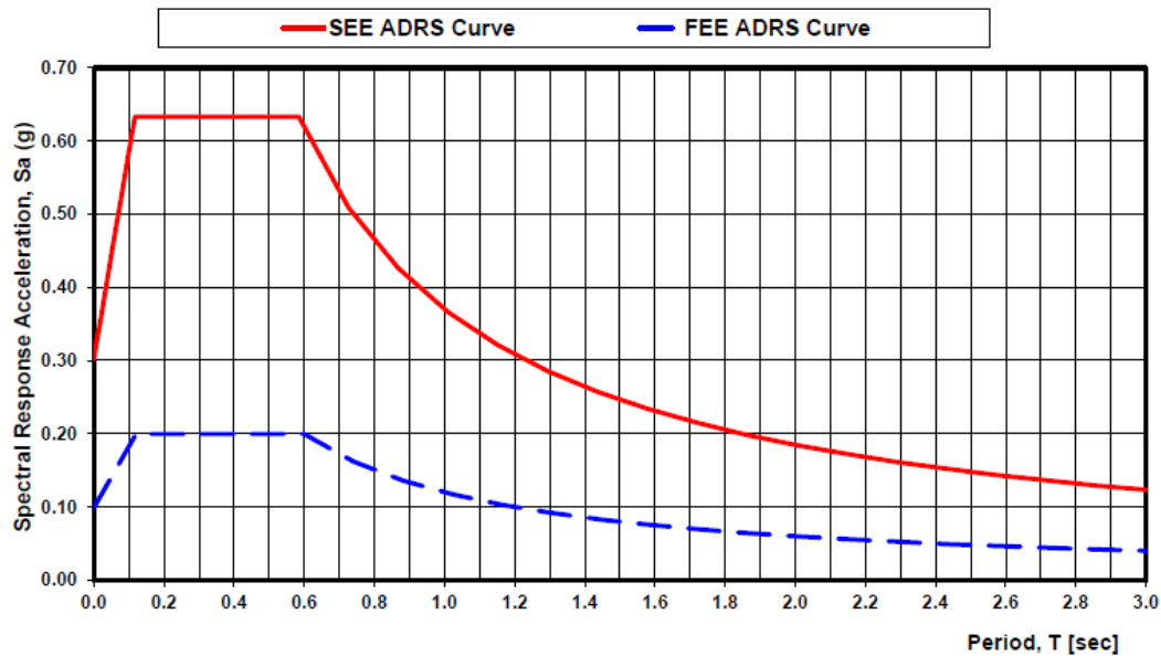
SC Seismic Hazard Map Three-Point ADRS Curve From Ground Surface, SC 41 - Site Class D
