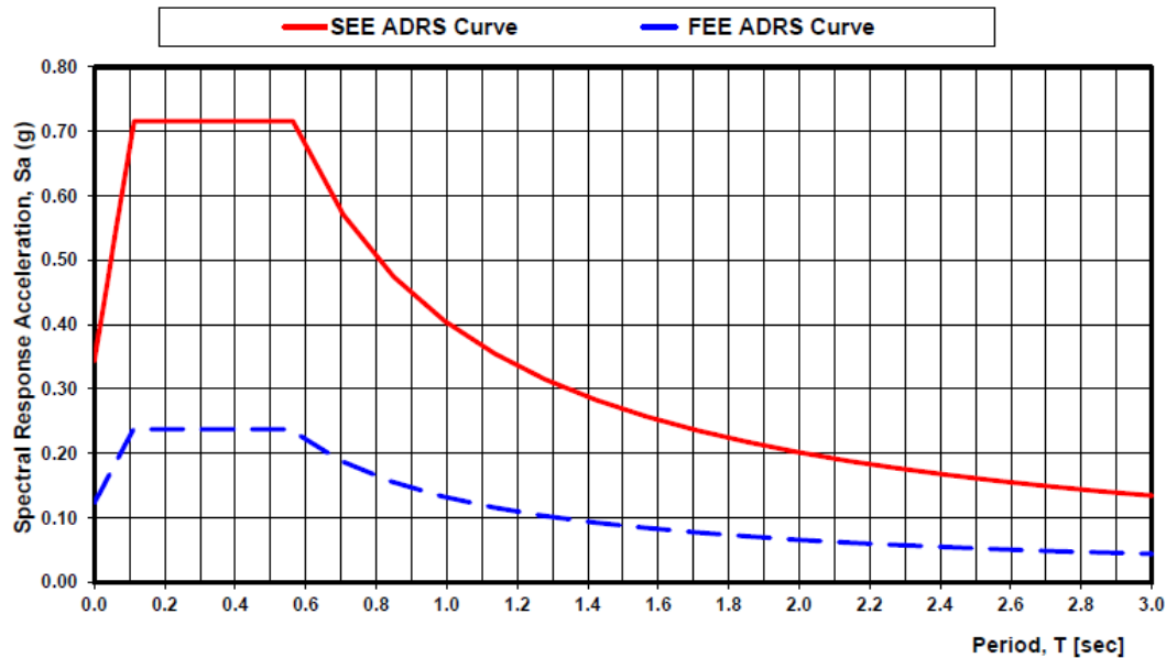
SC Seismic Hazard Map Three-Point ADRS Curve From Ground Surface, S-13 - Site Class D
