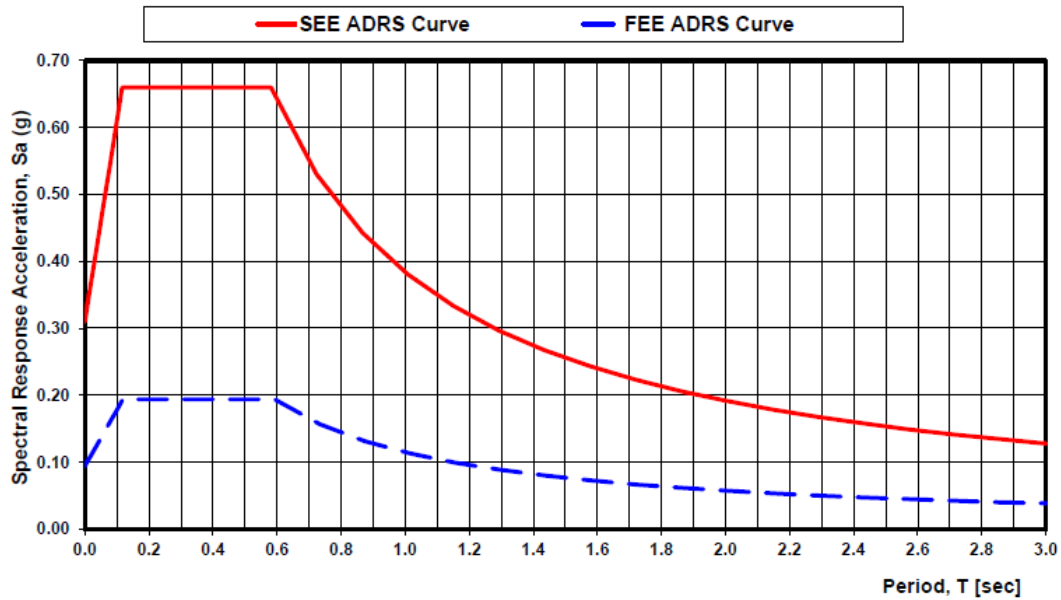
SC Seismic Hazard Map Three-Point ADRS Curve From Ground Surface, S-19 - Site Class D
