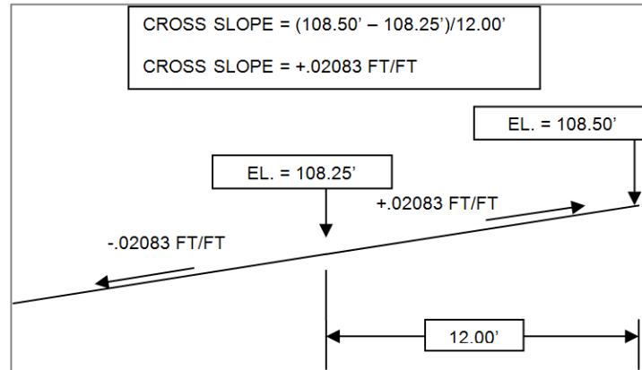
Figure 2 Remove Crown
