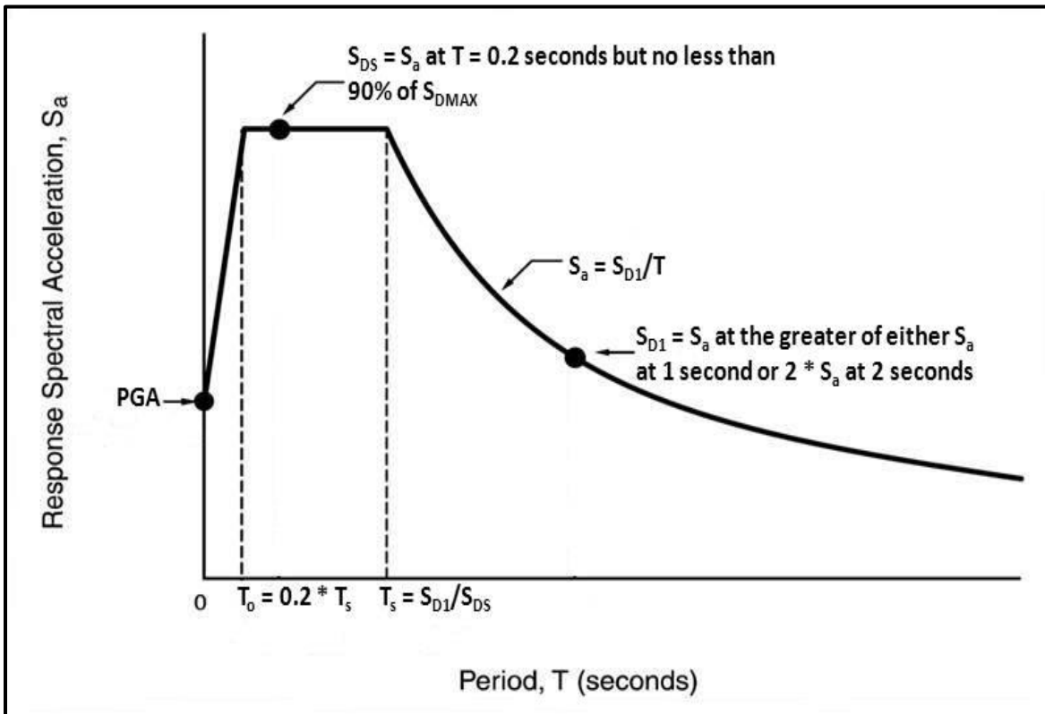
Figure 12.38, Site-Specific Horizontal ADRS Curve Construction
